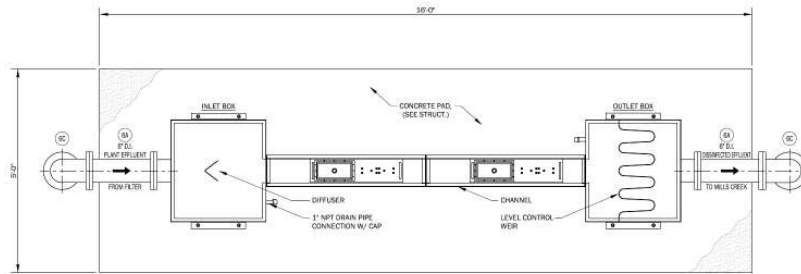
PLAN VIEW
