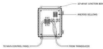
JUNCTION BOX DETAIL NO SCALE
