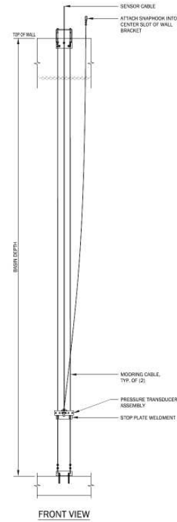
PRESSURE TRANSDUCER DETAILS NO SCALE
