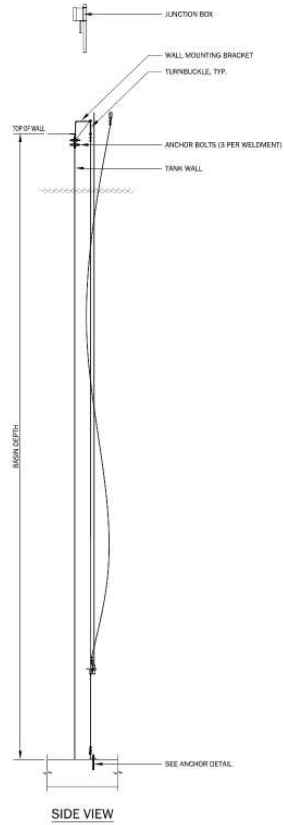
PRESSURE TRANSDUCER DETAILS NO SCALE
