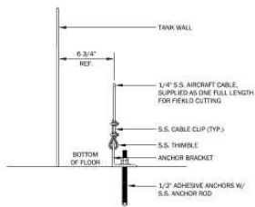
SUSPENSION CABLE ANCHOR DETAIL NO SCALE
