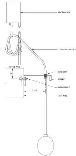
FLOAT SWITCH DETAIL NO SCALE
