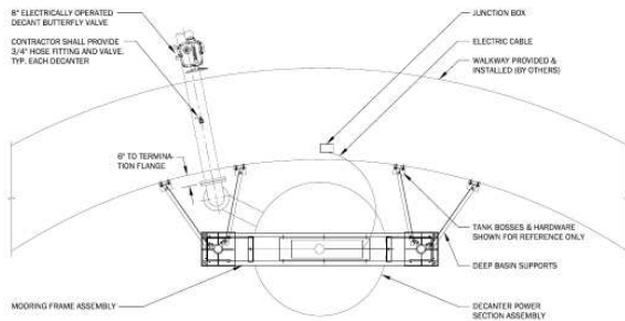
TANK ATTACHMENT PLAN VIEW
