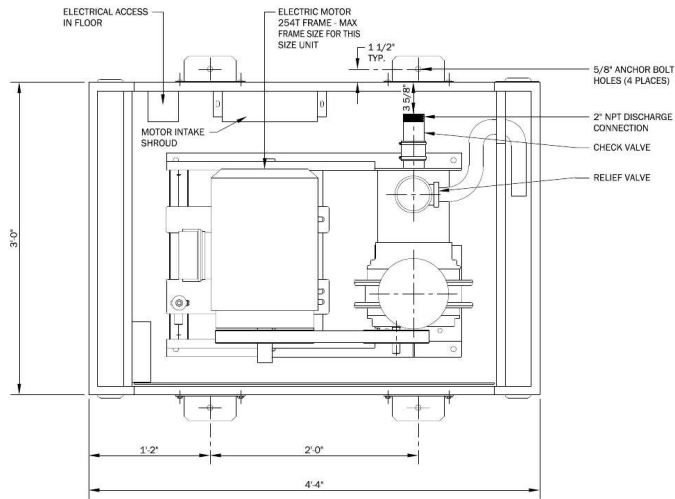
PLAN VIEW (TOP REMOVED)
