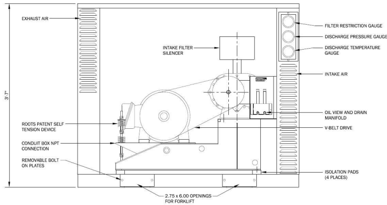
FRONT VIEW (FRONT PANEL REMOVED)
