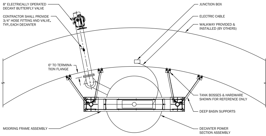
TANK ATTACHMENT PLAN VIEW
