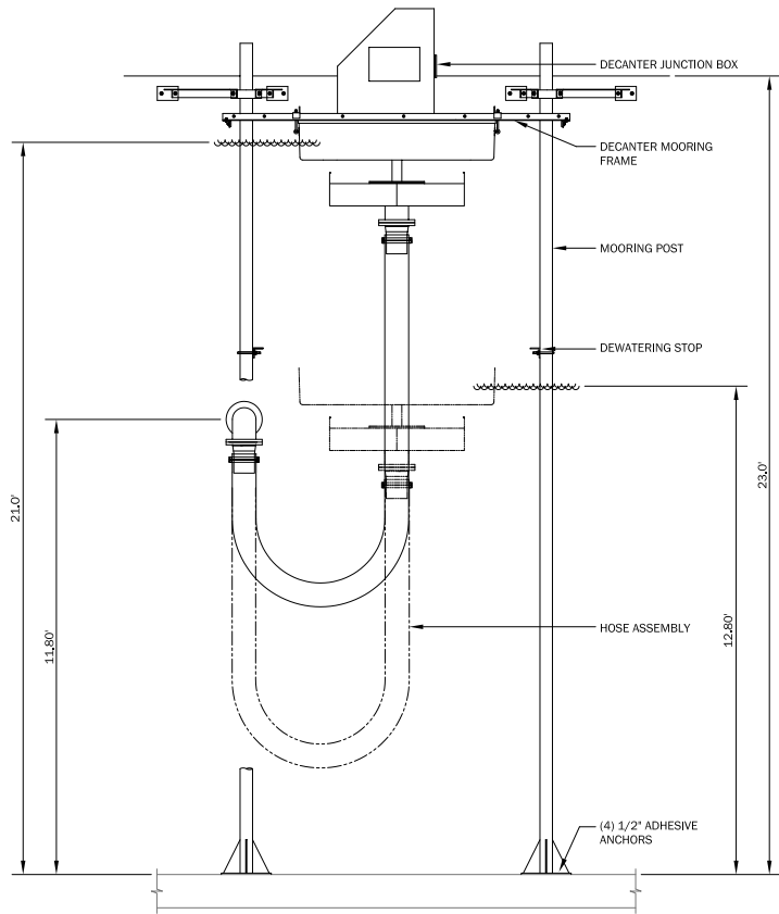
TANK ATTACHMENT ELEVATION VIEW
