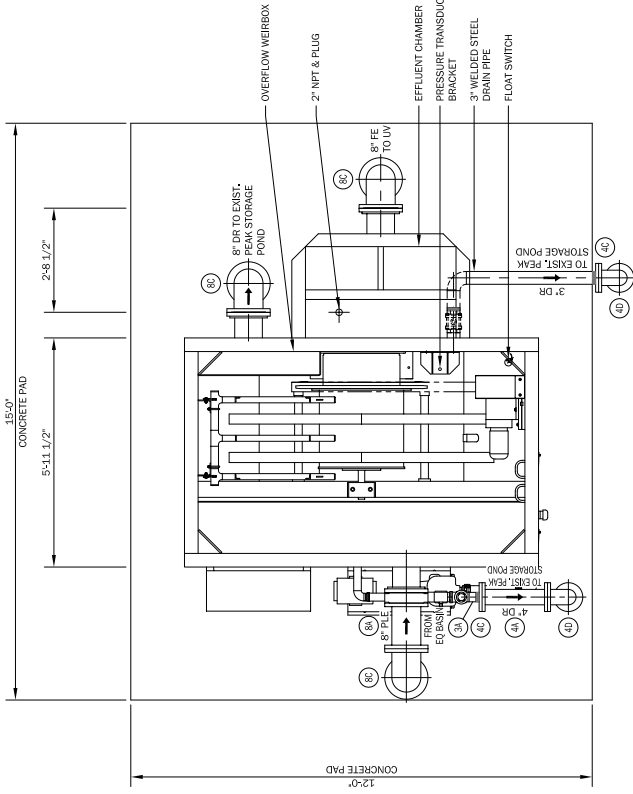
PLAN VIEW
