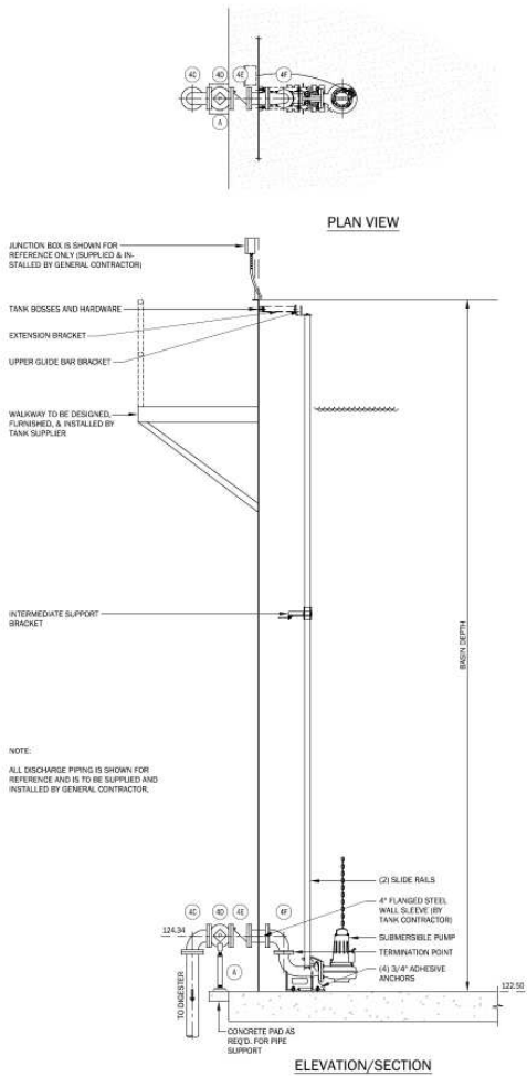
SBR TRANSFER PUMP DETAILS NO SCALE
