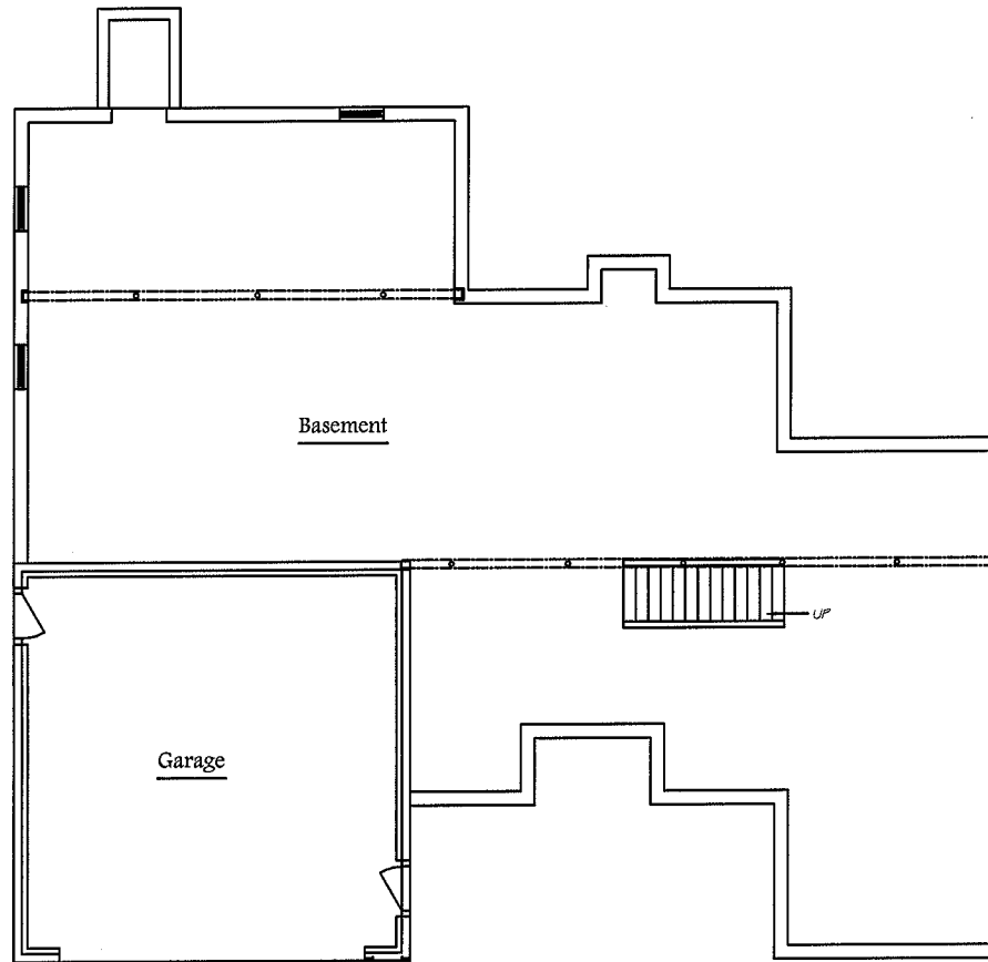
Basement Layout
