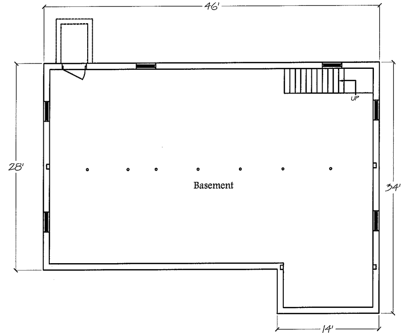
Basement Layout
