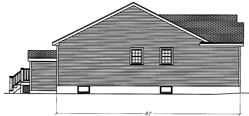
Left Elevation
