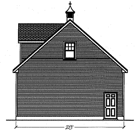
Rear Elevation
