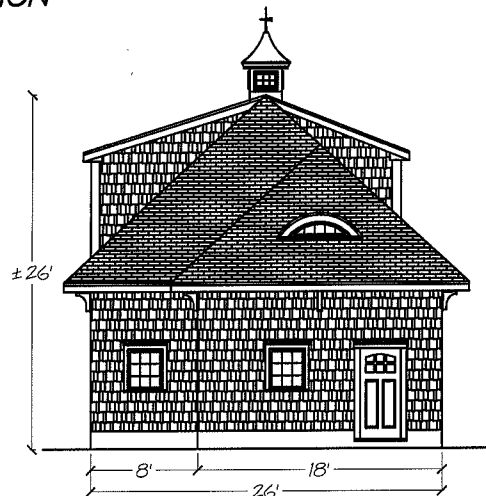
Left Elevation
