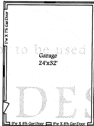
Floor Layout
