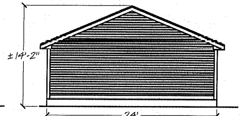
Rear Elevation
