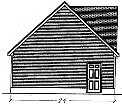
Left Elevation
