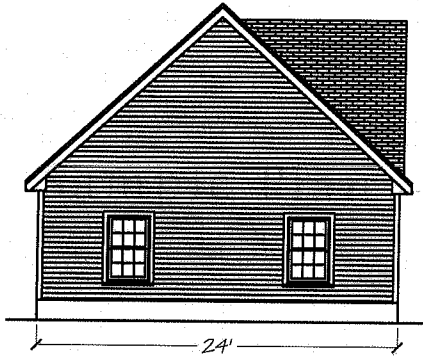
Left Elevation
