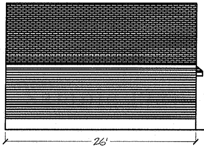
Left Elevation
