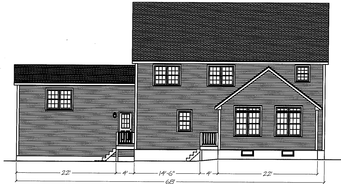
Rear Elevation
