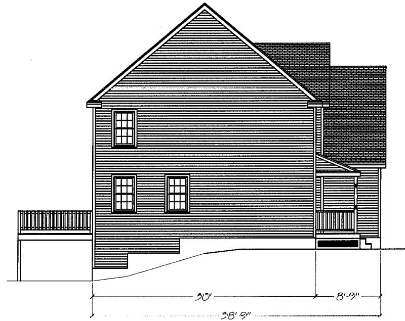
Left Elevation
