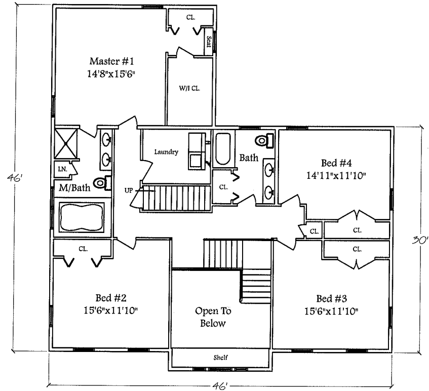
2nd Floor Layout
