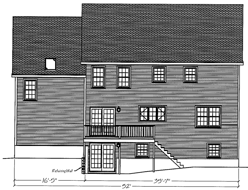
Rear Elevation
