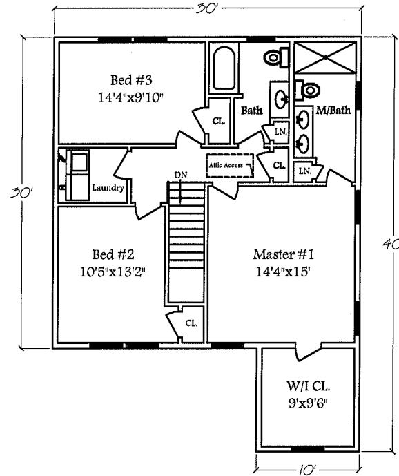
2nd Floor Layout
