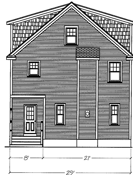
Rear Elevation
