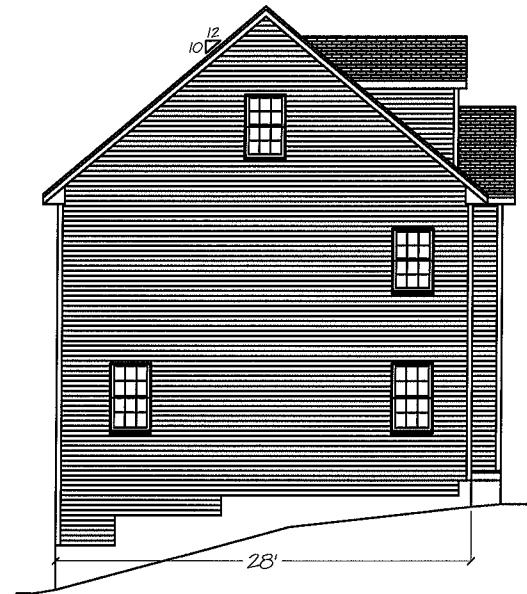
Left Elevation
