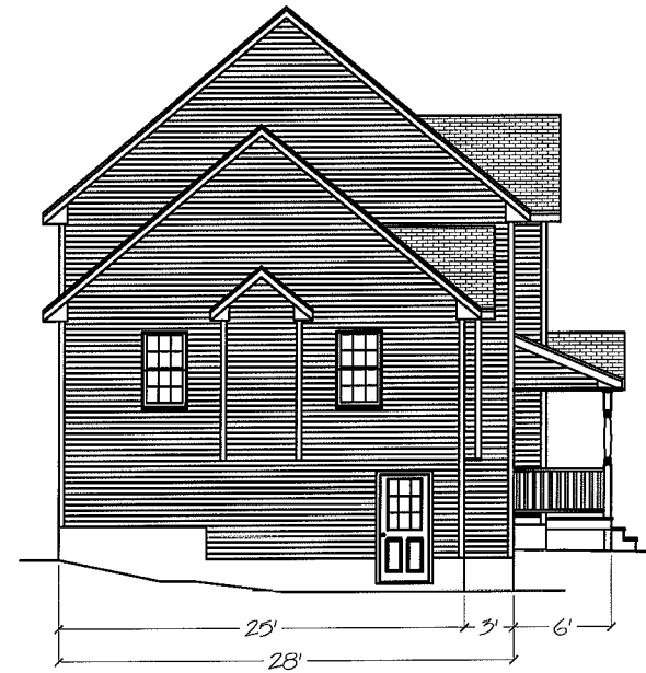
Left Elevation
