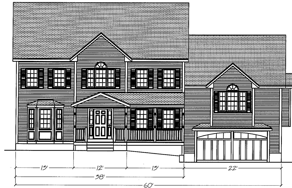
Front Elevation
