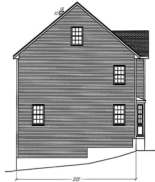
Left Elevation
