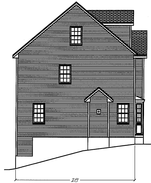
Left Elevation
