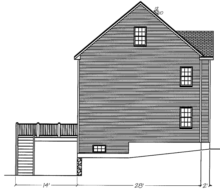
Left Elevation
