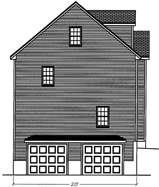
Left Elevation
