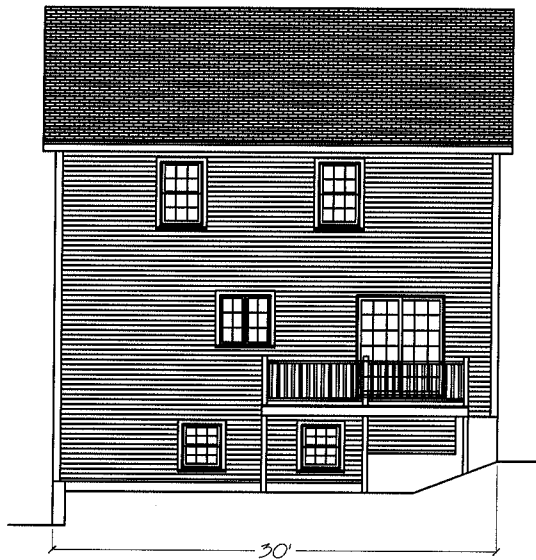
Rear Elevation
