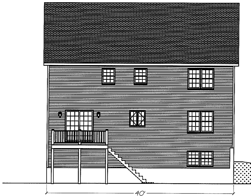
Rear Elevation
