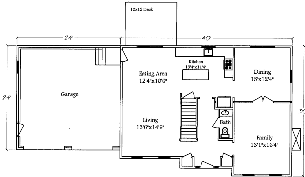
1st Floor Layout
