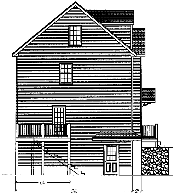
Left Elevation
