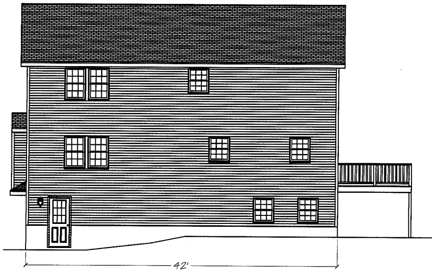
Rear Elevation
