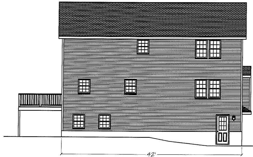
Rear Elevation
