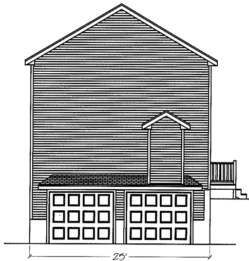
Left Elevation
