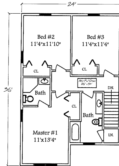
2nd Floor Layout
