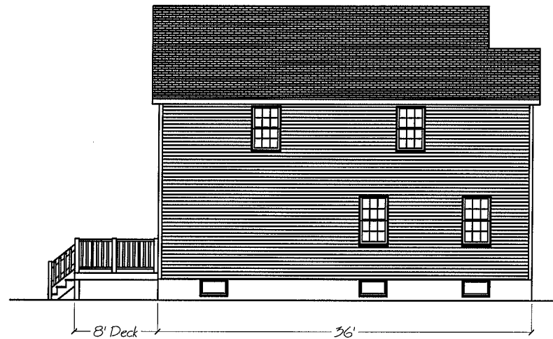
Left Elevation
