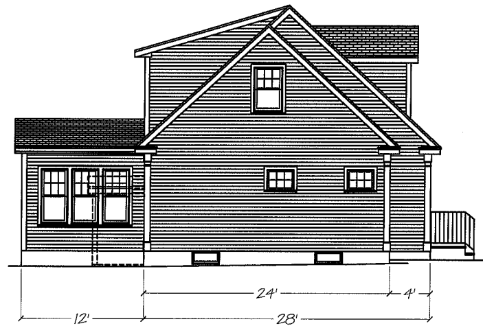
Left Elevation
