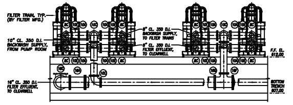
SECTION D-D SCALE 1/4" = 1'-0"
