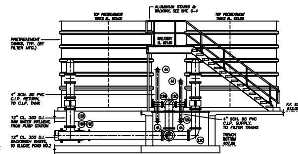
SECTION F-F SCALE 1/4" = 1'-0"
