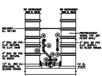
SECTION C-C SCALE 1/4" = 1'-0"
