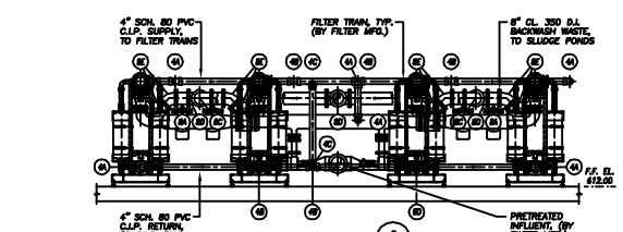
SECTION E-E SCALE 1/4" = 1'-0"
